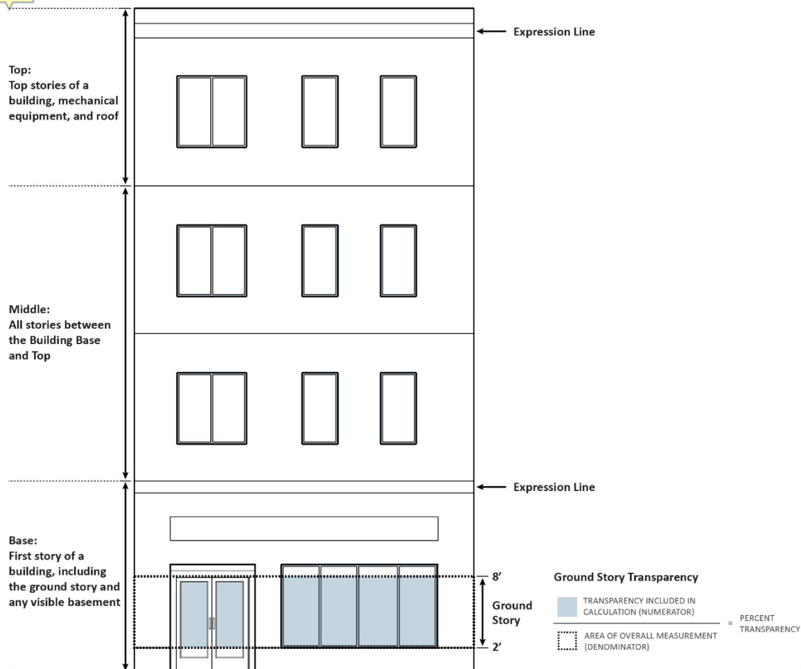
Figure 8.16.1 Business Districts Design Requirements: Front Elevation View
